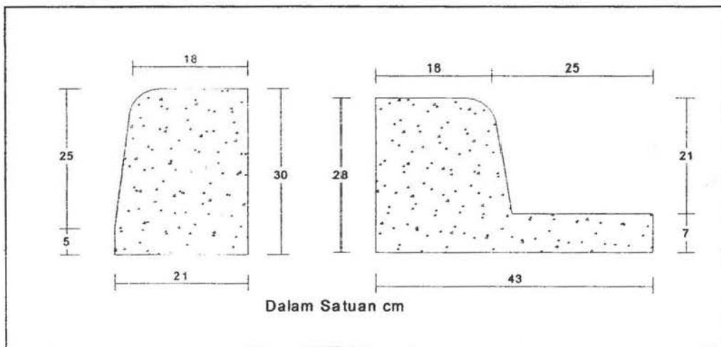
Gambar 5 Penampang melintang kereb
