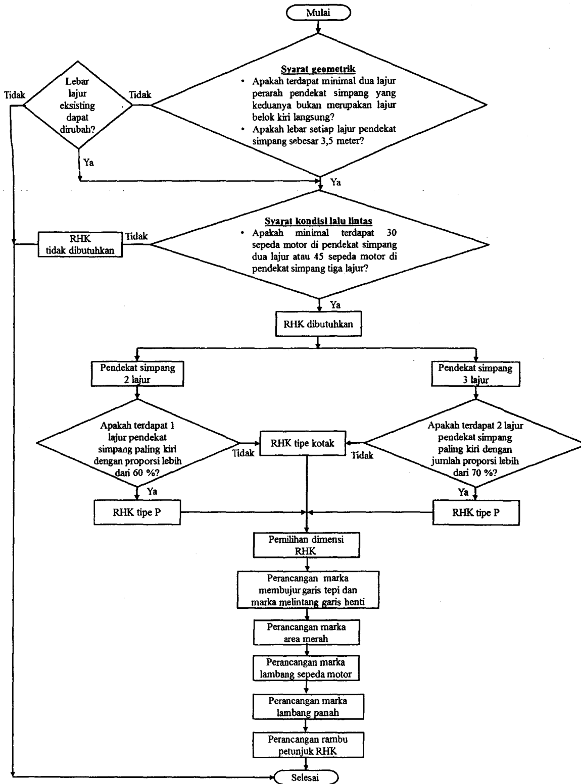
Gambar 19 - Prosedur perancangan RHK
