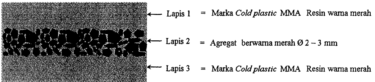
Gambar 14 - Detail A-A
