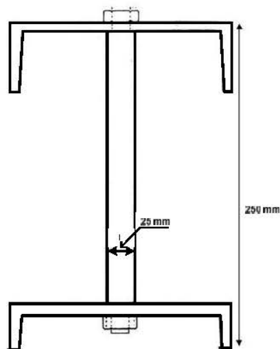
Gambar B.2 - Alat uji kohesi (tampak samping)
