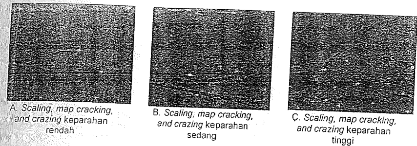
Gambar 40 - Tingkat keparahan scaling, map cracking, and crazing
