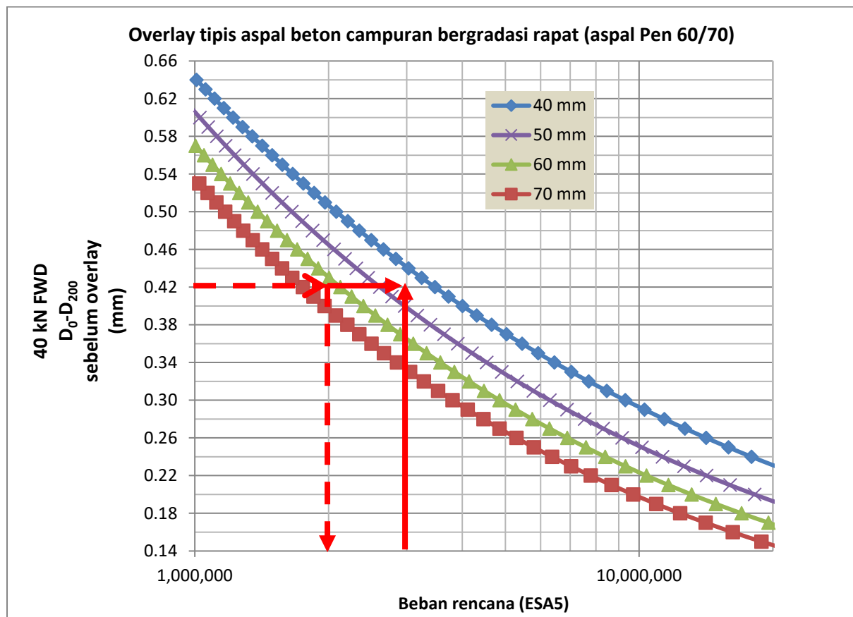
(a) Overlay tipis
