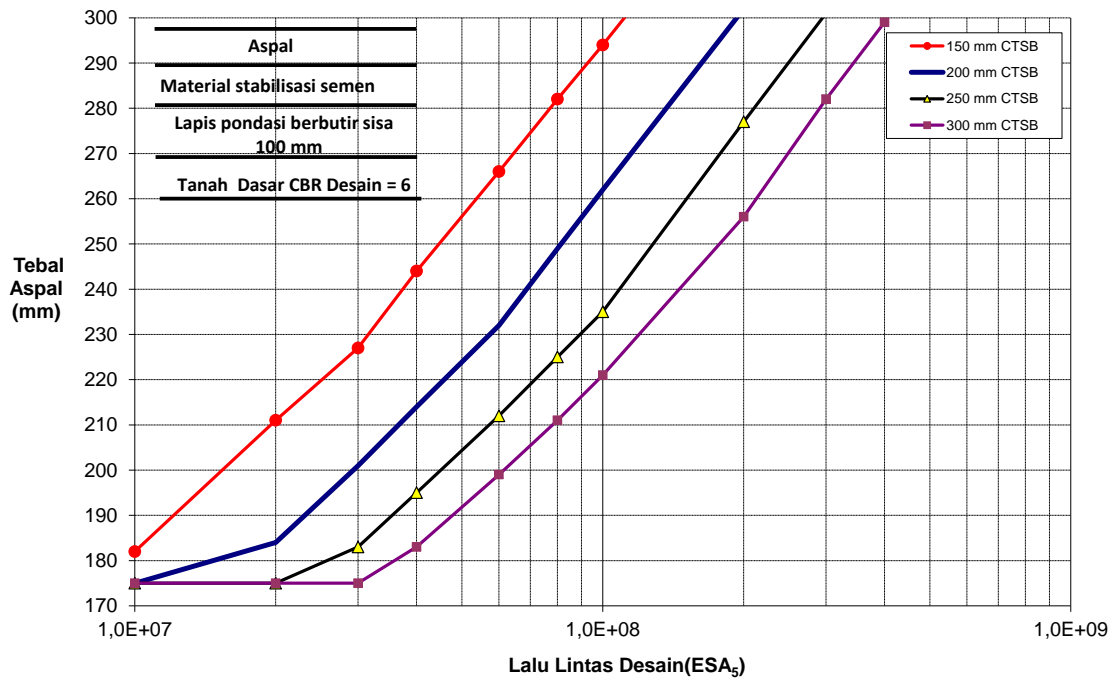
Gambar 8.4. Bagan Desain Ketebalan Cement Treated Recycled Base (CTR)
